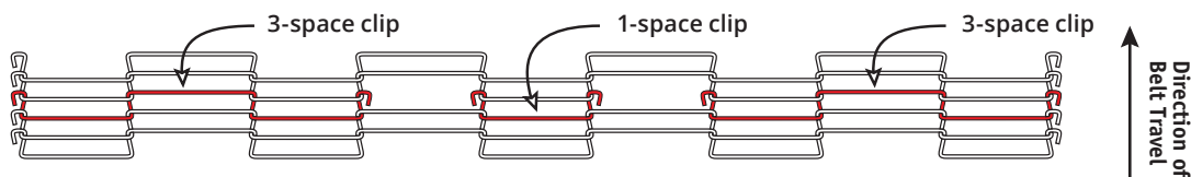
9-space single loop edge belt
