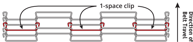
5-space single loop edge belt
